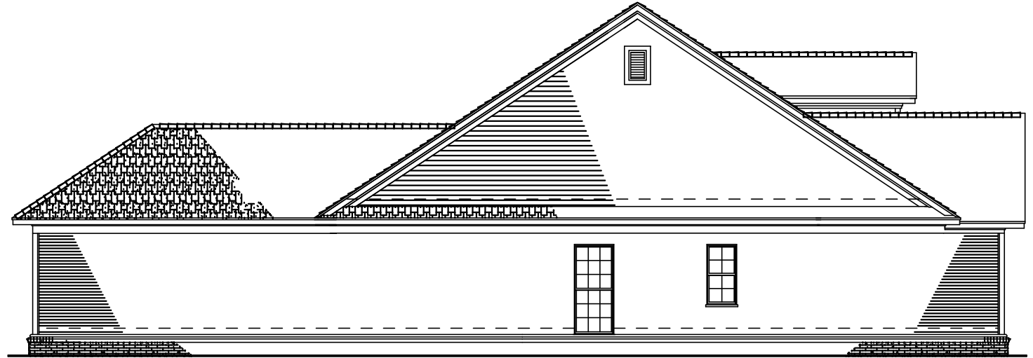
LEFT ELEVATION
